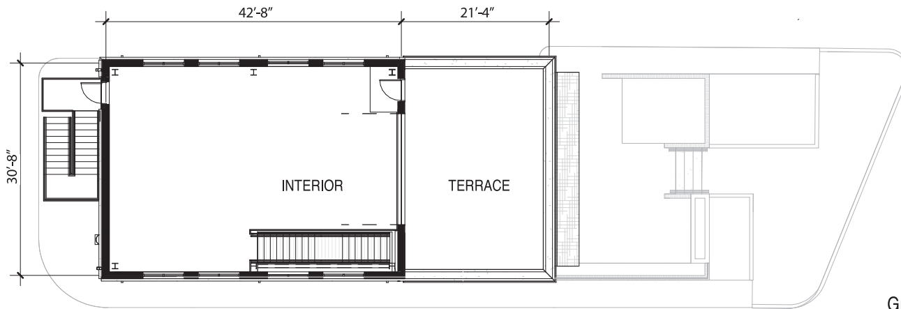
SECOND FLOOR LEVEL
